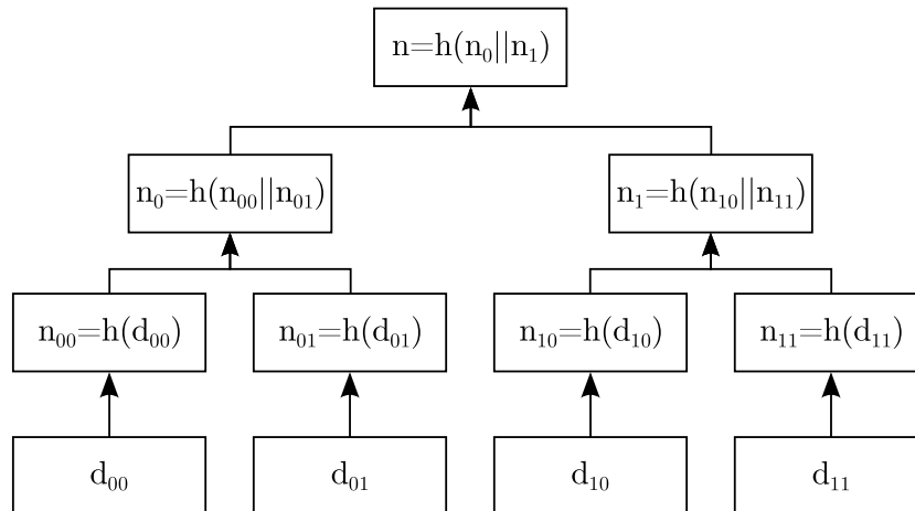
Figure 2.1. Merkle Tree
