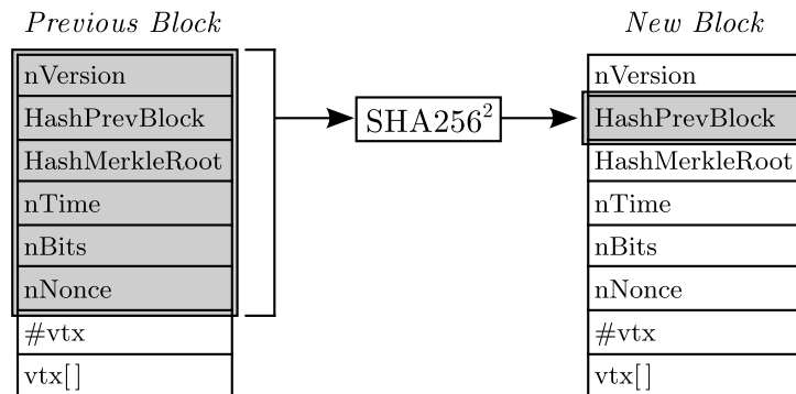
Figure 3.1. Block Reference Computation
